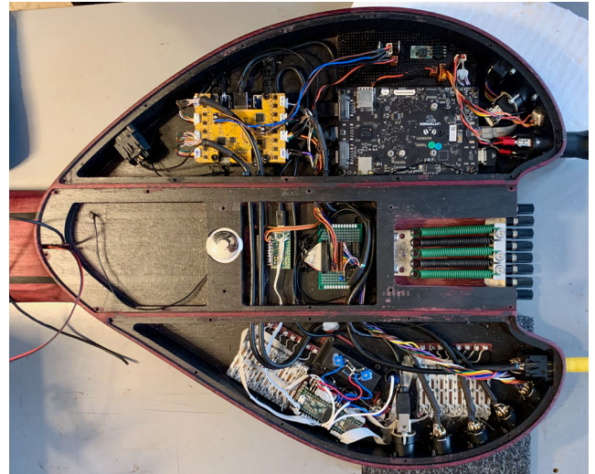
Figure 7: The electronics housed in the body of the Sophtar. The ADC/DAC board is on the top left (yellow), whilst the SBC is on the top right (black). The two Teensy microcontrollers are in the centre and bottom sections.
